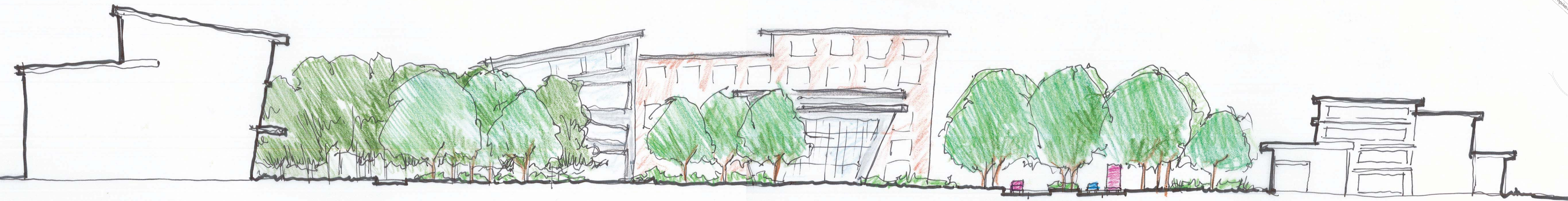
B - Institutional (Med / R+D Campus) Courtyard and Boulevard
